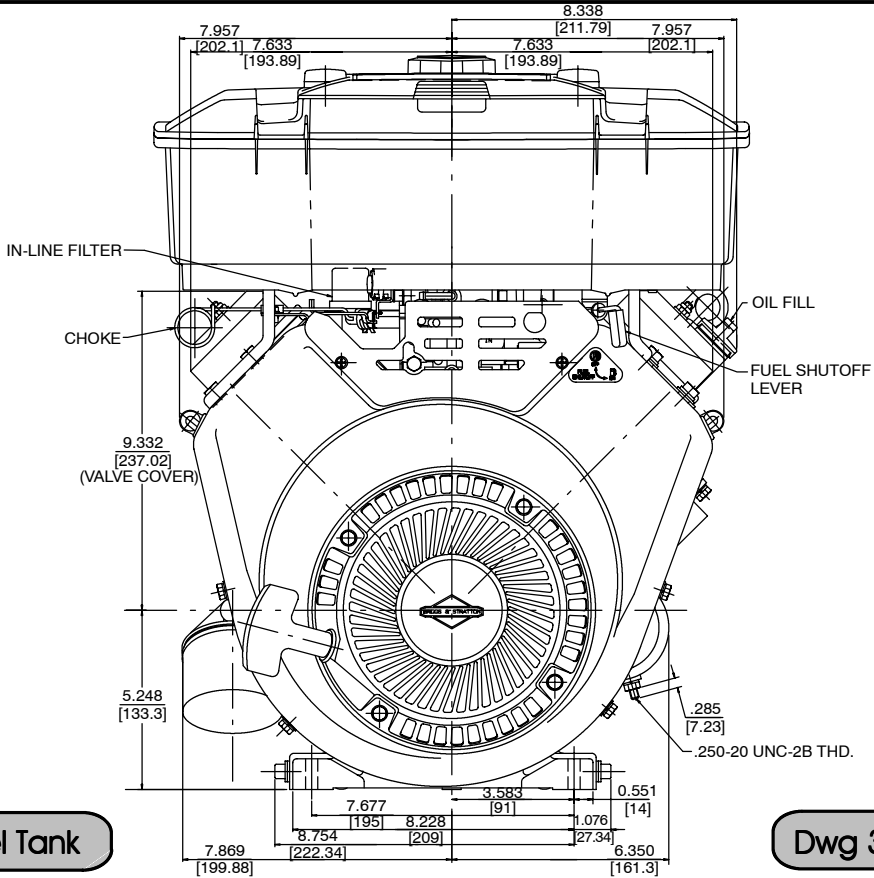
Dwg 350400000016
